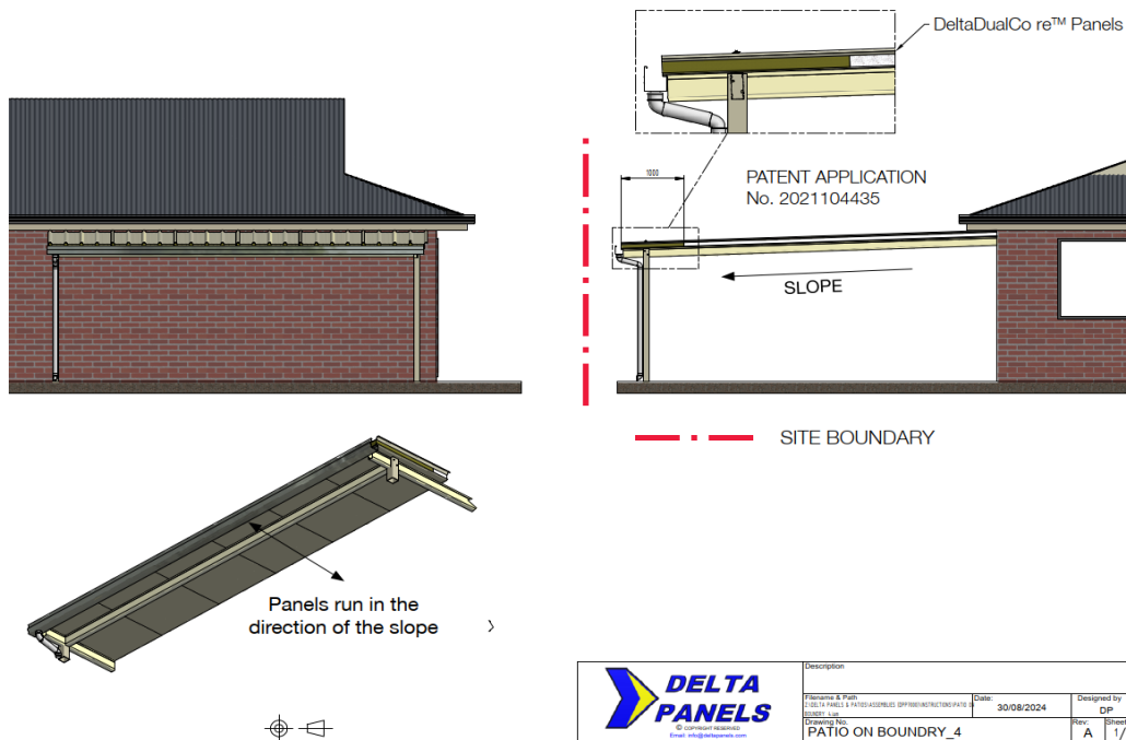
Figure 3-4. DeltaDualCore™ system sloping towards the site boundary.
